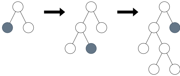
FIGURE 3. Leaf-wise tree growth in LightGBM.
